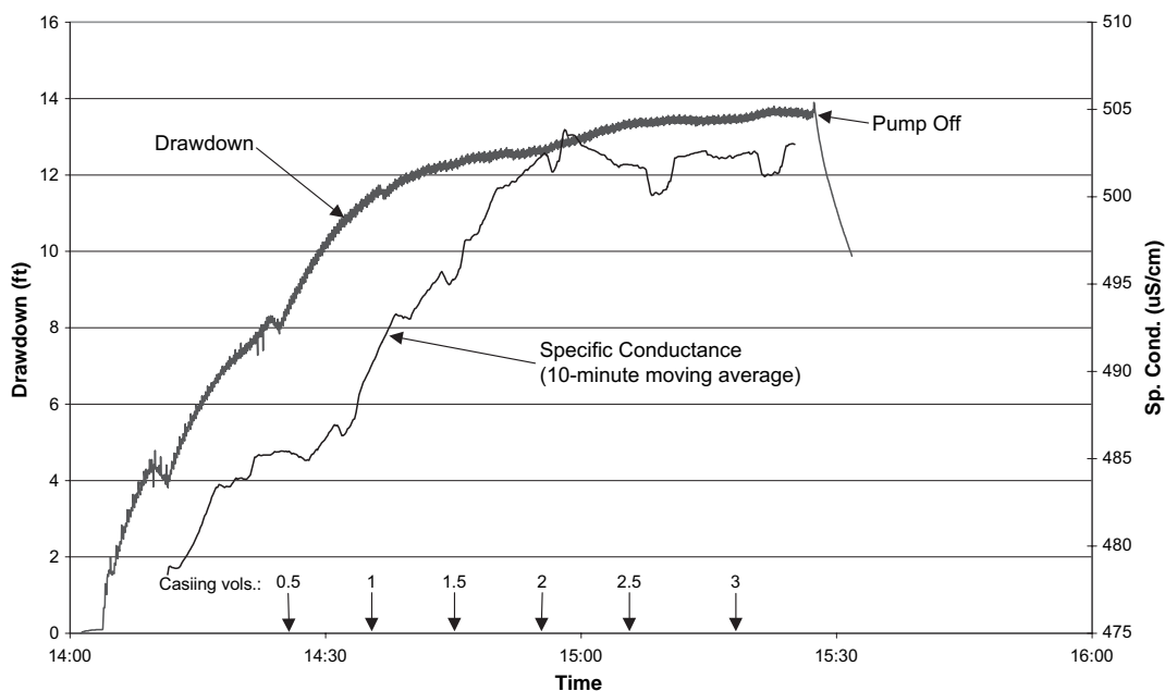
Figure 1. Drawdown and specific conductance during purging well D-2A.
